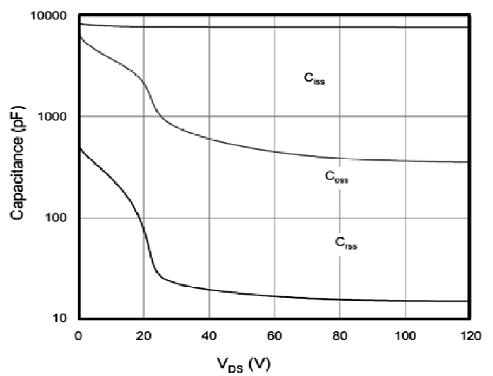
Capacitance
