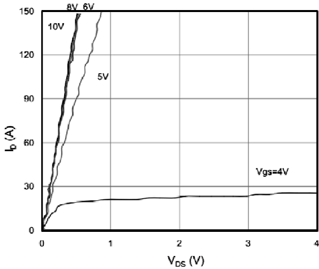
Output Characteristic
