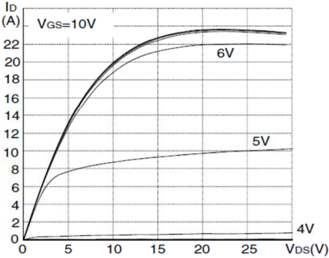
Output Characteristic
