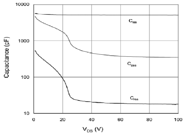
Capacitance
