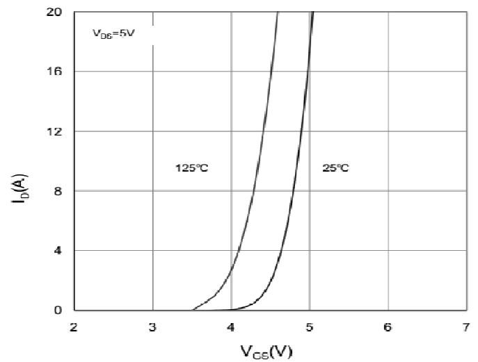
Transfer Characteristic
